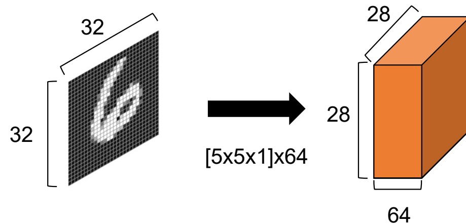
5x5 Convolution layer (#weights: 1,600)
